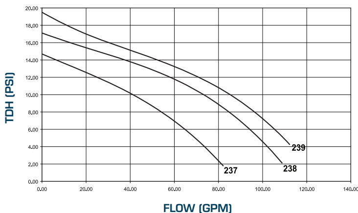
50Hz PERFORMANCE CURVE Export International Model
