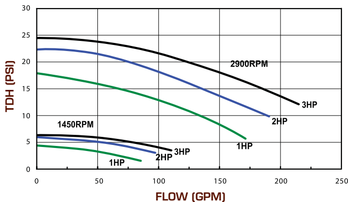
50Hz PERFORMANCE CURVE International Model
