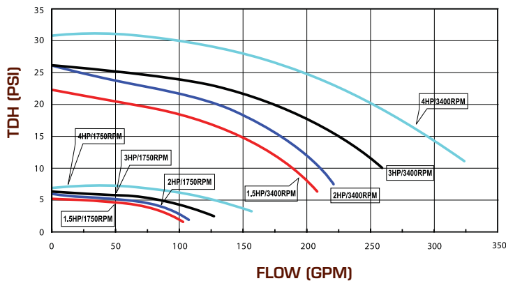
60Hz PERFORMANCE CURVE North America Model
